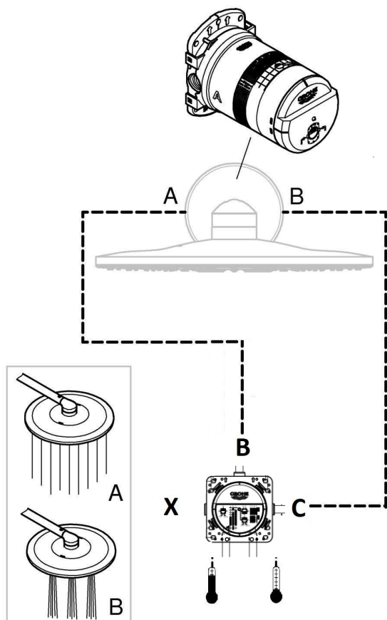
Above illustration shows Grotherm SmartControl 2 button model
